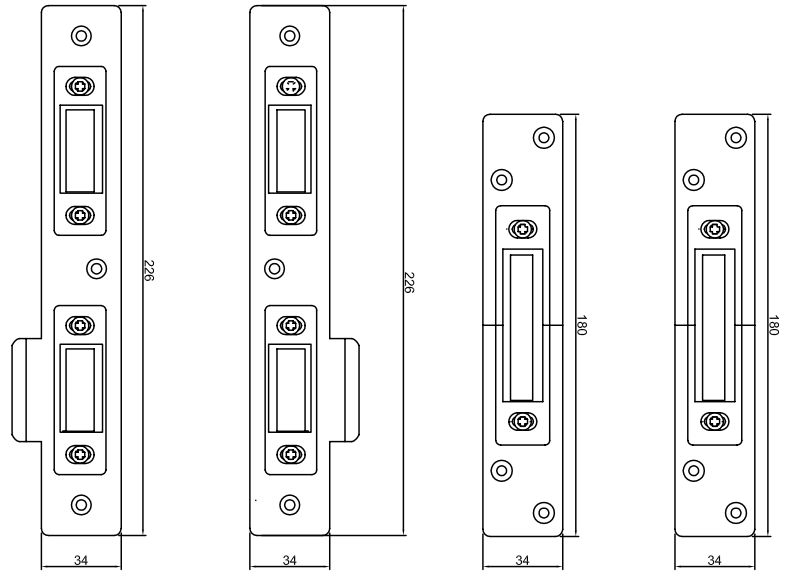
XLC0001-KE Centre Keep
