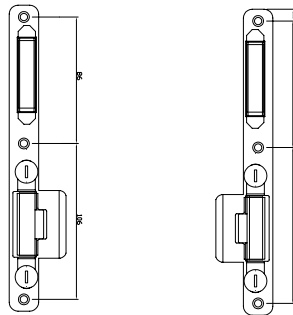
CRB0014-KE CENTRE KEEP LEFT HAND
