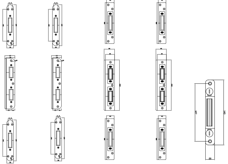
CRB0005-KE FULL SET HOOK KEEP Non handed
