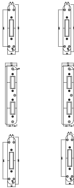
CRB0005-KE FULL SET HOOK KEEP Non handed
