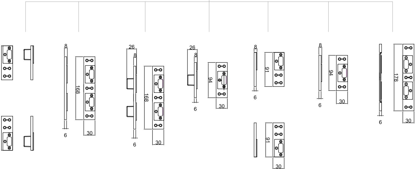
XLKBR SB Single door shoot bolt keep
